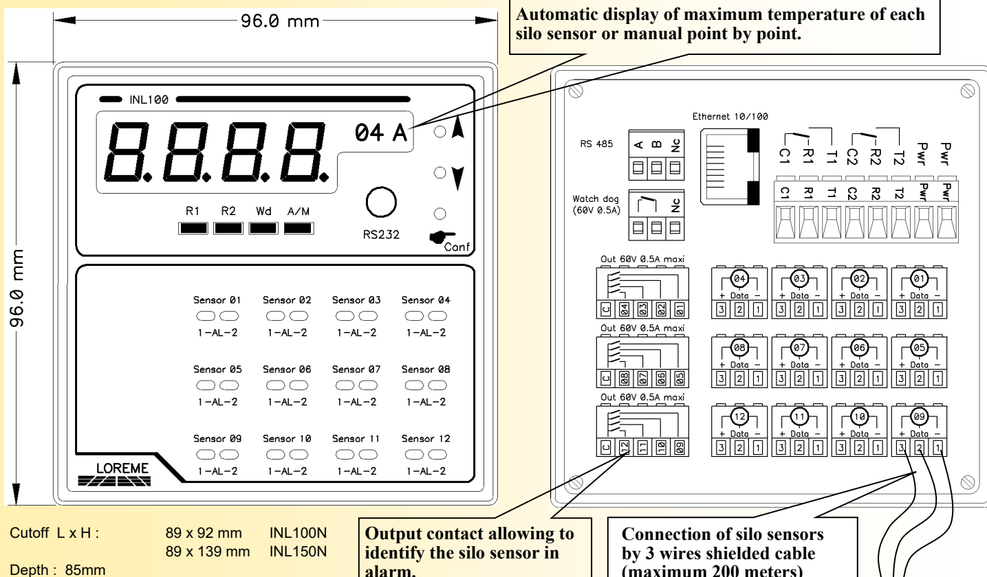
Digital Silo Sensor Siloflex-N Type of maximum 24 temperature points
