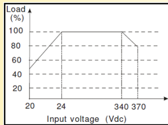
Output power function of input voltage
