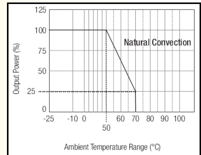
Output power characteristics vs ambient temperature
