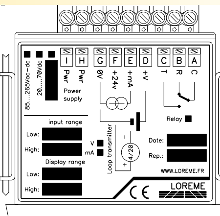
Version entrée 4..20mA / 0...10V
